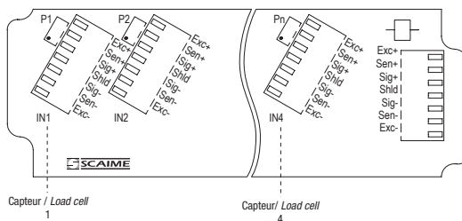
Carte raccordement 4 capteurs - 4 load cells junction board
