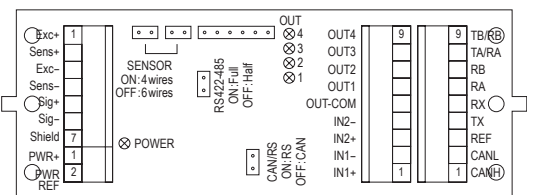
Carte eNod3 - eNod3 board
