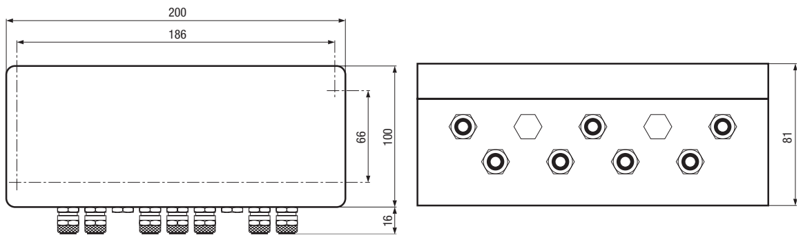
Carte raccordement 4 capteurs - 4 load cells junction board
